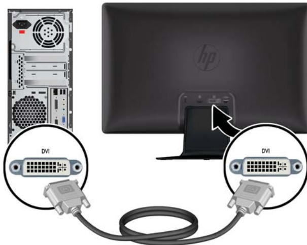
Figure 3-4 Connecting the DVI-D Cable (cable provided with select models only)
